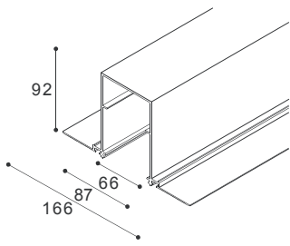
Recessed Track
