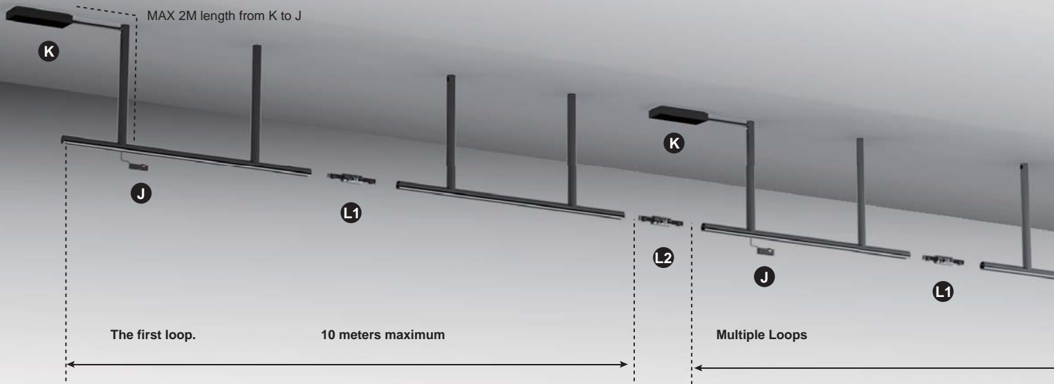
TT connection illustration
