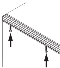
Secure the profile with screw, the height of the screw head shall not exceed 2mm.
