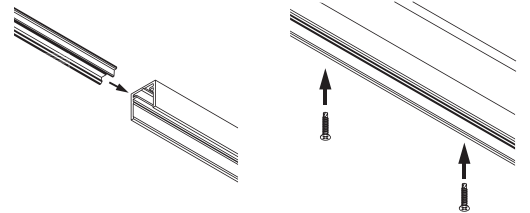
Pre-drill 7mm holes on the aluminum profile, secure the profile with screws on the surface, the height of the screw head shall not exceed 2mm.
