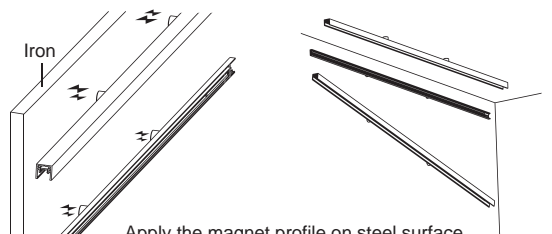
Apply the magnet profile on steel surface.
