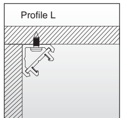
Secure the profile with screw, the height of the screw head shall not exceed 2mm.
