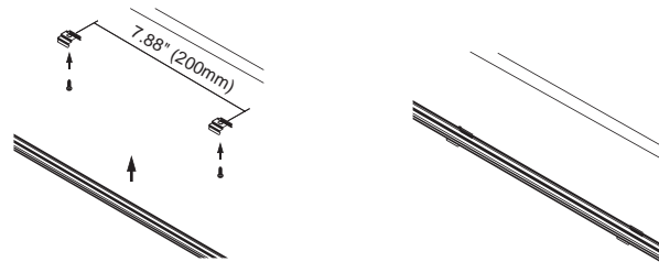
Distance between clips is 200mm, secure the clips with screw then click the track on the clips.
