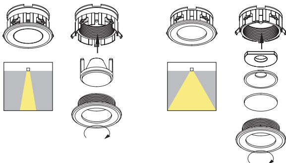
optic lens 36°
