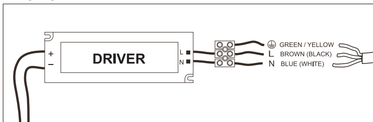
Wiring diagram
