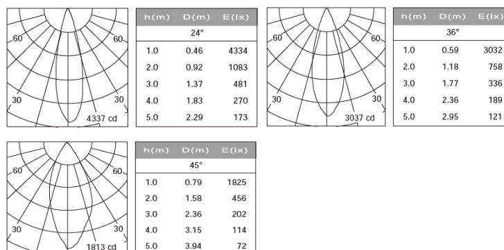
ACHO-4 Honeycomb louver
