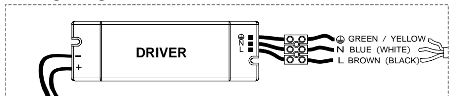
Wiring diagram
