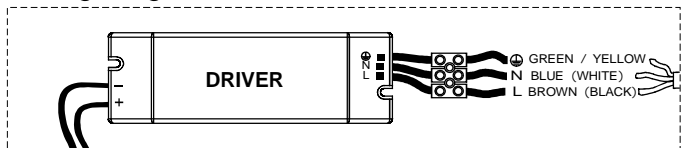
Wiring diagram
