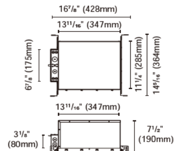
ACCH-7B-100-PUP40A-1WMC-850 0/1-10V ACCH-7B-100-PUP40D-1WMC-850 DALI ACCH-7B-100-PUP40T-1LMC-850 TRIAC for BRANKO-B-110-3.5" (30W) Type: IC Box
