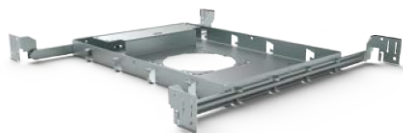
ACCH-12H-100 for BRANKO-B-110-3.5" Type: New construction plate
