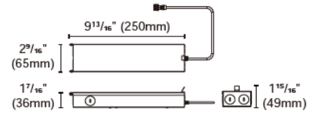
ACCG-16B-PUP40A-1WMC-850 0/1-10V ACCG-16B-PUP40D-1WMC-850 DALI ACCG-16B-PUP40T-1LMC-850 TRIAC for BRANKO-B-110-3.5" (30W) Type: Gear box
