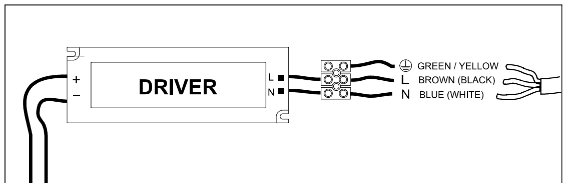
Wiring diagram
