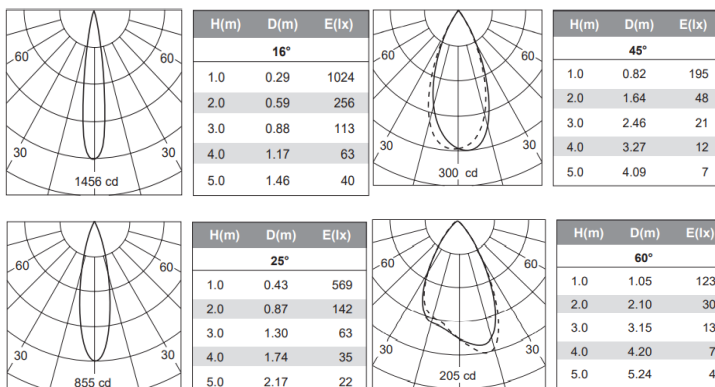
DS-005 Diffusers
