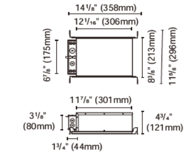
ACCH-12B-100-PUP20A-1WMC 0/1-10V ACCH-12B-100-PUP20D-1WMC DALI ACCH-12B-100-PUP20T-1LMC TRIAC for BRANKO-A-110-3.5" (20-21W) Type: IC Box
