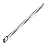
Models : CLC-12A 40"(1000mm) Models : CLC-12B 197"(5000mm) Type : Singal wire connect to system / dimmer
