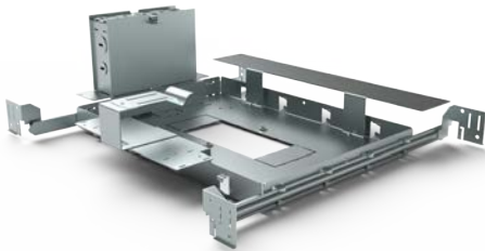
ACCH-12L-61X181-EM for STAR Multiple Type: NON-IC New construction plate with emergency battery holder
