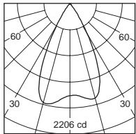
2018.495-LEA15DW 2018.295A-LEA15DW
