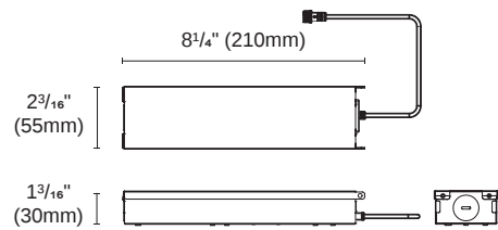
ACCG-20A-LBS12W-16-C0700-RD for 4T ACCG-20A-LBS12W-16-C0600-RD for 5T ACCG-20A-LBS30W-42-C0600-RD for 10T ACCG-20A-LBS30W-48-C0550-RD for 15T ACCG-20A-PSB50W-0850-56 for 15TW
