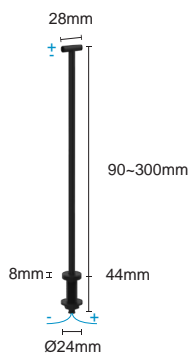
DIVA8-POLE-TA2 T pole
