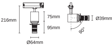
Framing 2319.210F-UA-350
