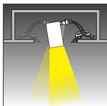
Dual channel recessed slot
