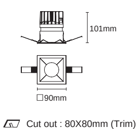
Cut out : 80X80mm (Trim)
