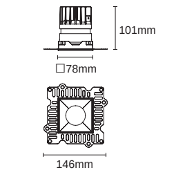
Cut out : 82X82mm (Trimless)
