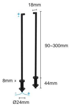
DIVA8-POLE-LA2-CV DIVA8-POLE-LA2-CC Linear pole
