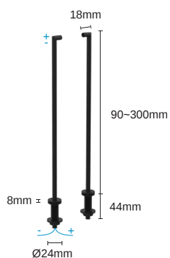
DIVA8-POLE-LA2-CV DIVA8-POLE-LA2-CC Linear pole
