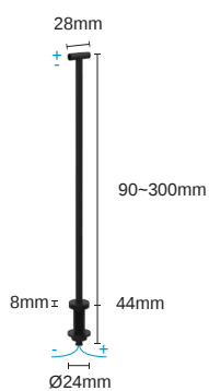
DIVA8-POLE-TA2-CV DIVA8-POLE-TA2-CC T pole
