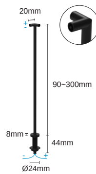
DIVA8-POLE-CA2-CV DIVA8-POLE-CA2-CC Corner pole
